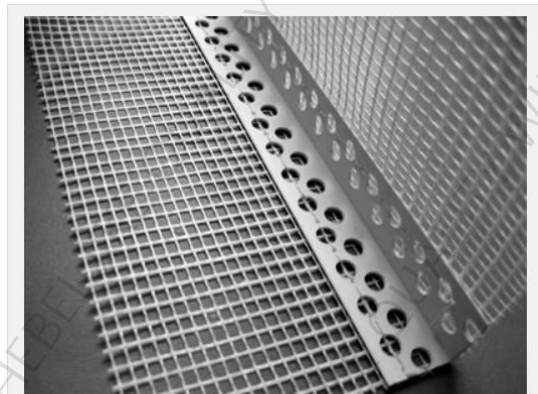
PVC bead with fiberglass mesh helps to improve the reinforcement and offer heat preservation effect, also diverse colors offered.
